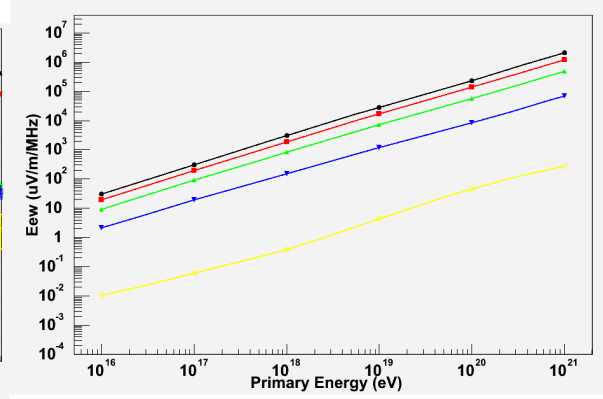
Figure 4: East-west 10MHz signal component vs. primary energies, 24 showers average out shower-to-shower fluctuations at each energy with signals and measured as in figure 3, the fitted power-law slopes are 0.96, 0.95, 0.94, 0.92 and 0.80.
